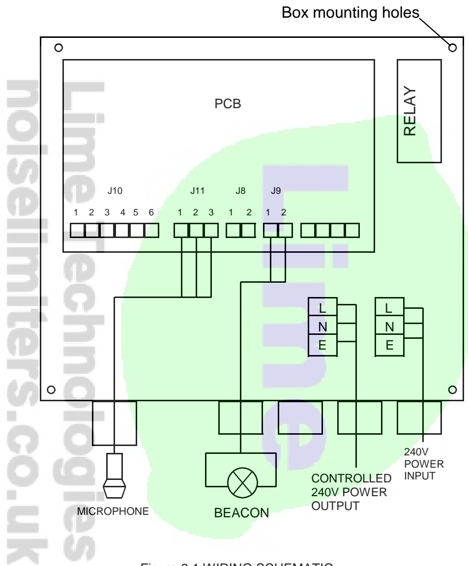
Figure 3.1 WIRING SCHEMATIC
